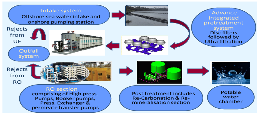
Figure : 1 : Overview of R.O Process
